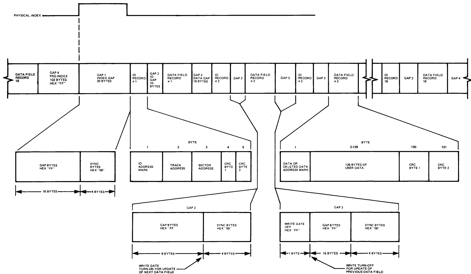
FIGURE 21. TRACK FORMAT-18 RECORD/TRACK
