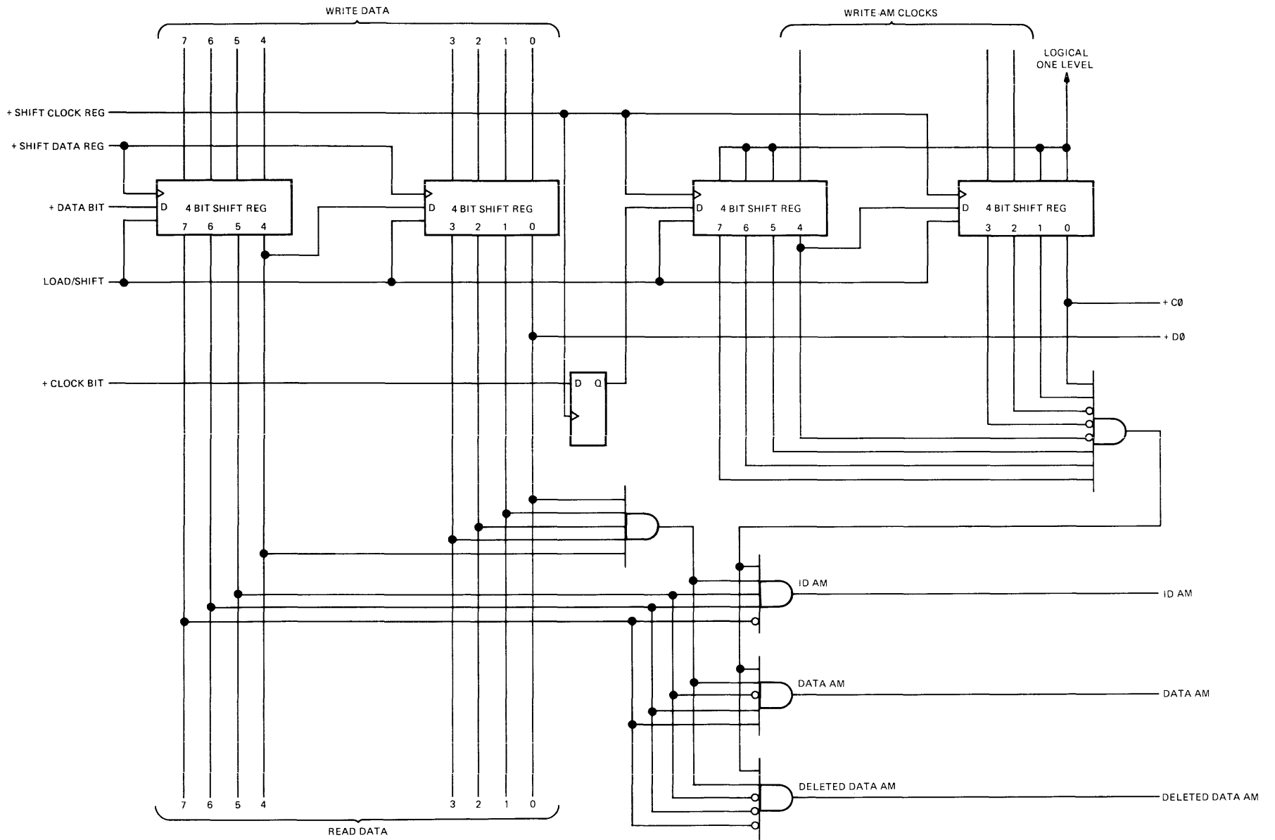
FIGURE 31. DATA AND CLOCK REGISTERS
