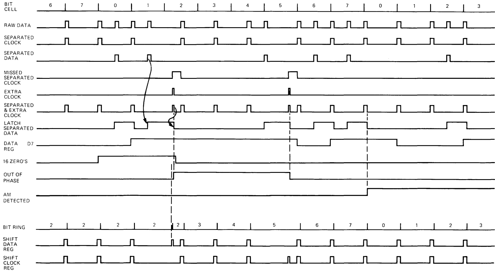
FIGURE 32. AM TIMING
