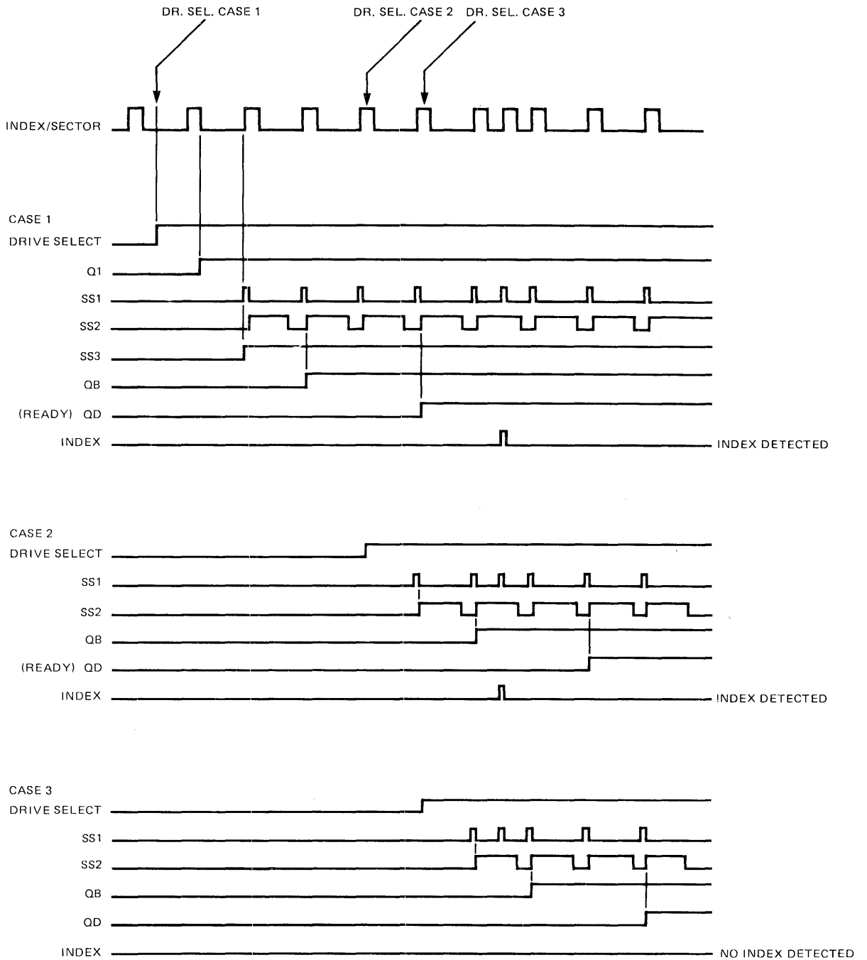
FIGURE 35. INDEX/SECTOR TIMING
