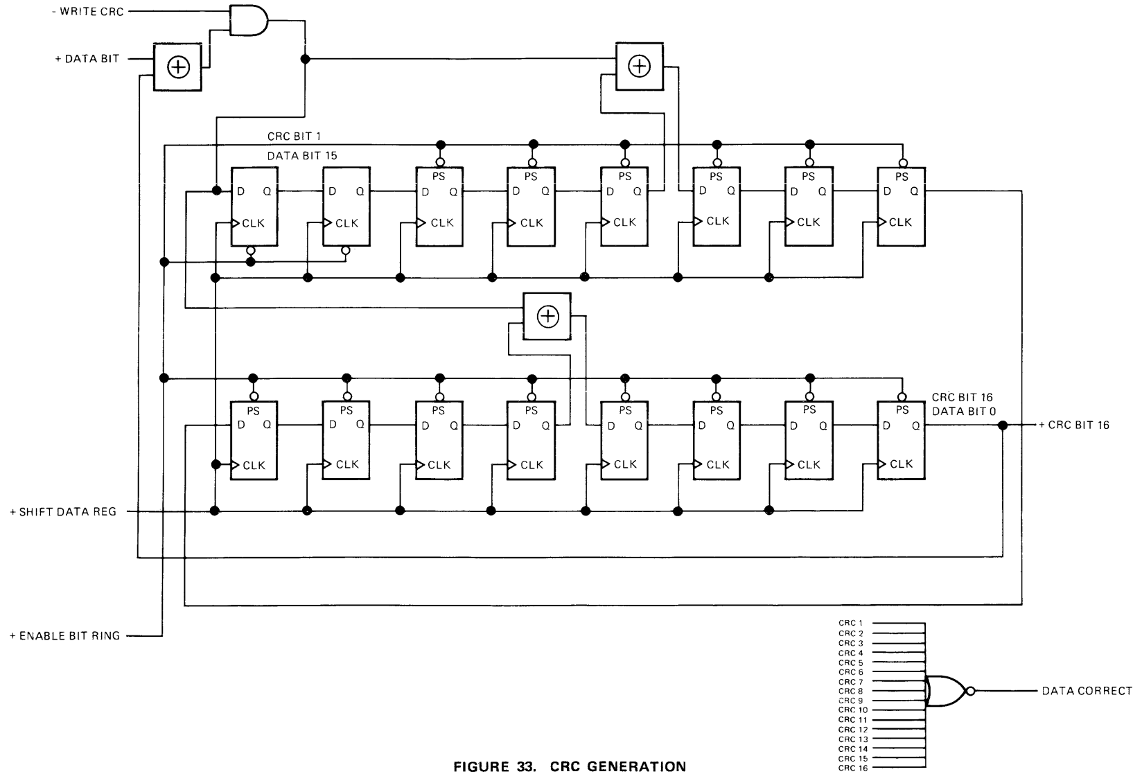
FIGURE 33. CRC GENERATION
