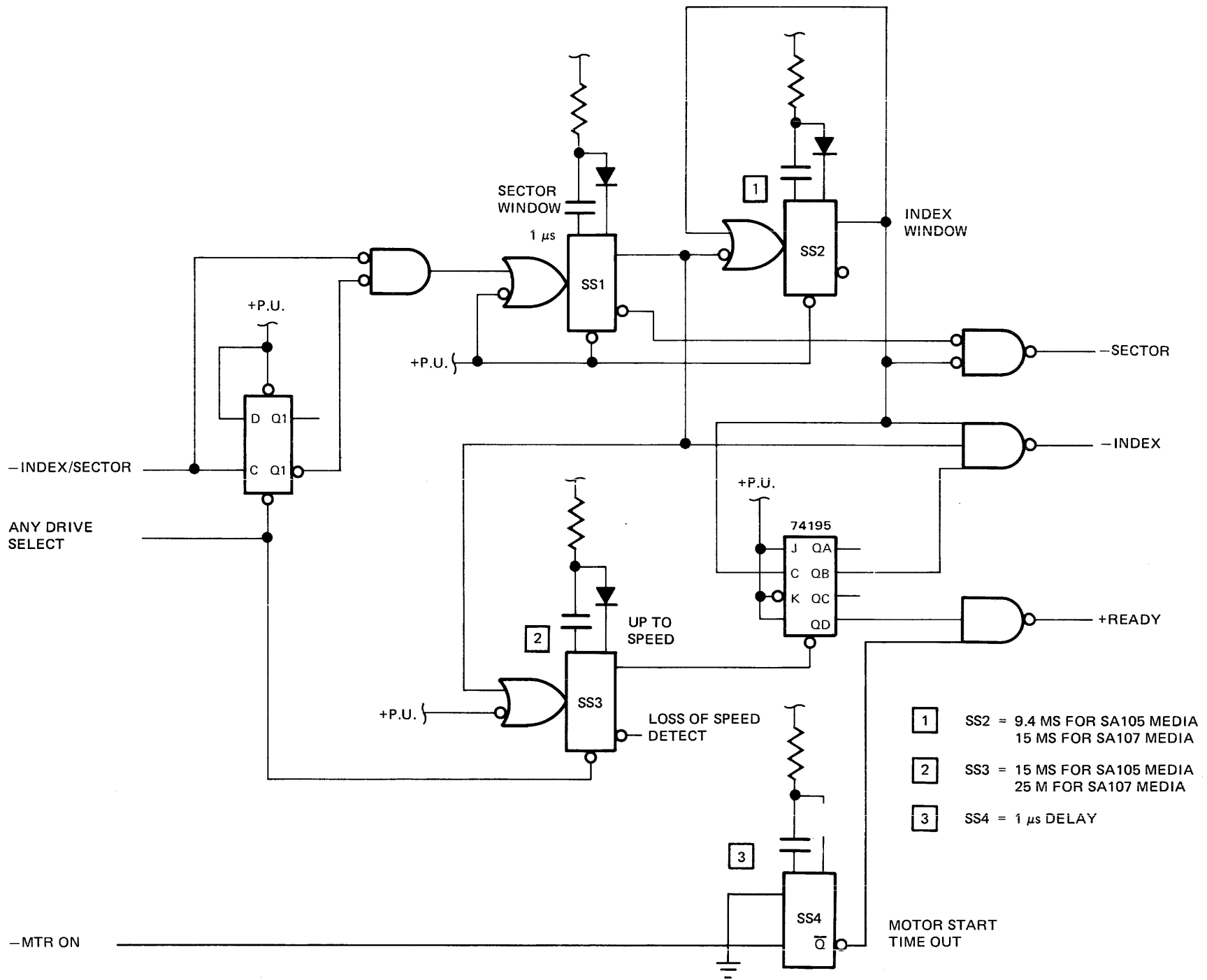
FIGURE 34. INDEX/SECTOR SEPARATOR AND READY CIRCUIT
