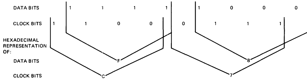
FIGURE 24. DELETED DATA ADDRESS MARK
