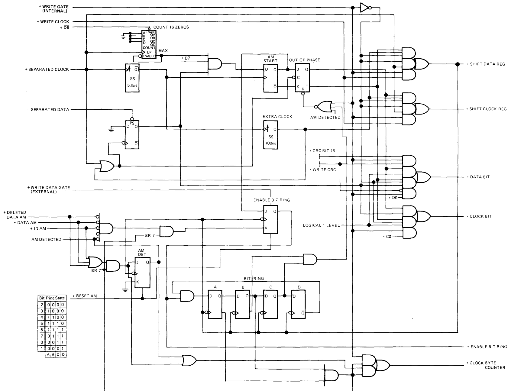
FIGURE 30. REGISTER CONTROLS AND AM DETECTION
