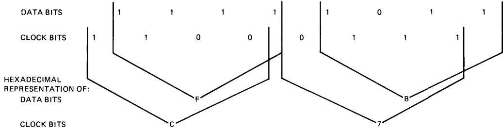
FIGURE 23. DATA ADDRESS MARK
