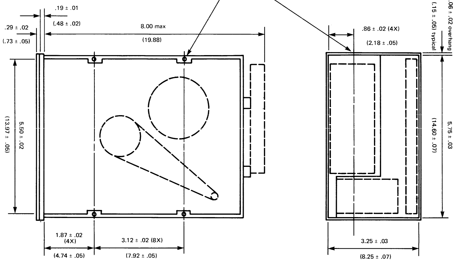
FIGURE 16. SA400 DRIVE DIMENSIONS
