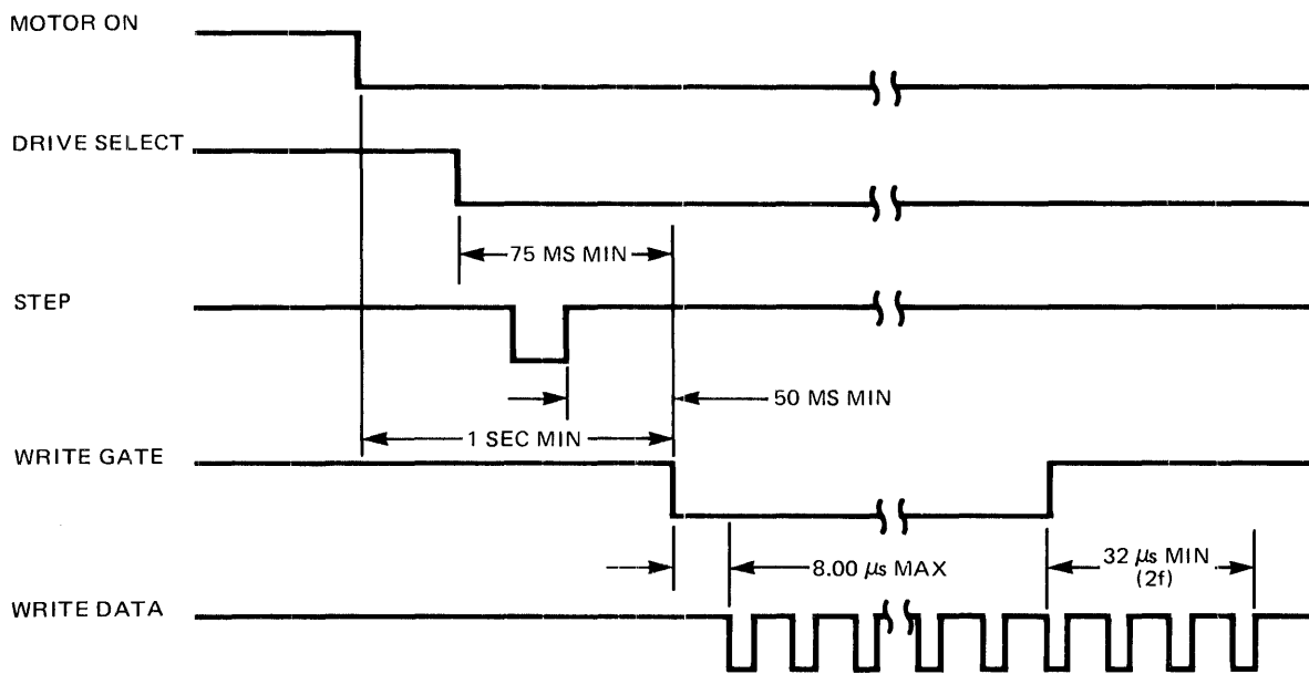
FIGURE 6. WRITE INITIATE TIMING
