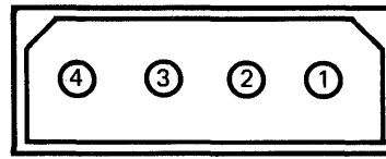
FIGURE 14. J2 CONNECTOR
